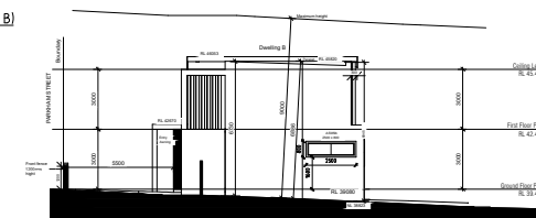
WESTERN ELEVATION (LOT B)
